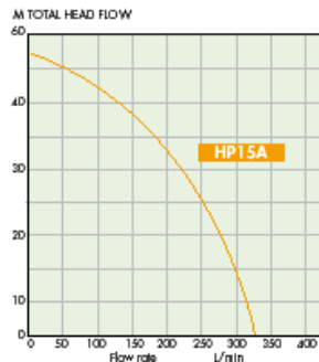
Performance Curves
